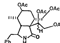
22 , β-H
