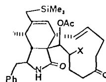
15 , X = SCH 3
